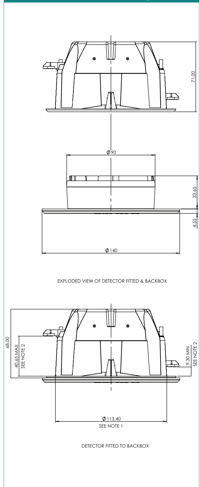
Figure 1: Soteria Dimension Optical Detector dimensional drawing
