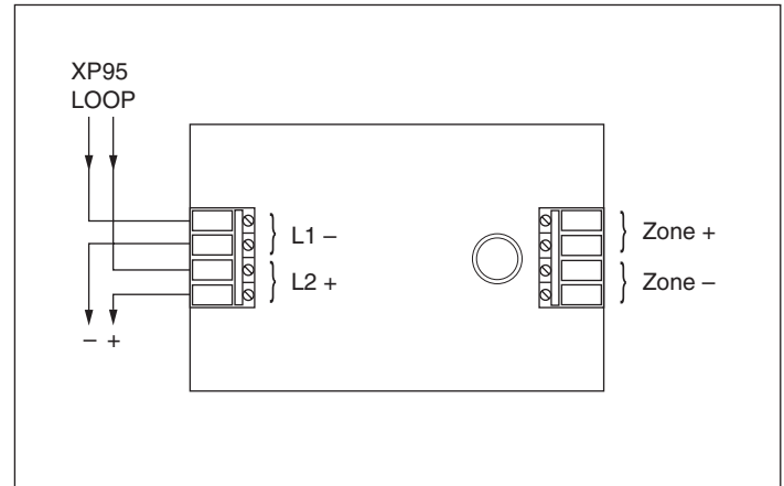
Fig.1 Loop connections
